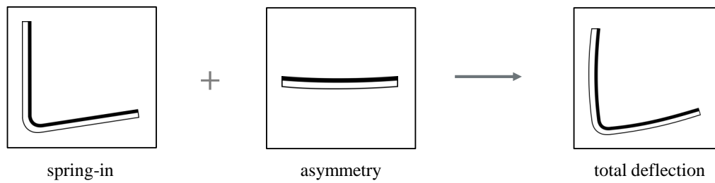
Figure 4: The total deflection of RTM-parts is driven by two main underlying mechanisms: spring-in and asymmetry. As representation for possible asymmetries and V_f -gradients in thickness-direction, neat resin layers on L-shaped CFRP-specimens are investigated.
