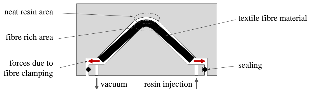
Figure 2: Schematic of fibre bridging effect and immersion edge tool: In a typical state of the art closed mould RTM-process fibre clamping may lead to in-plane tensional forces in the preform. As a result the fibre bridging effect develops. After the resin injection process a fibre rich area close to the inner radius occurs (convex tooling side) whereas at the outside a resin rich area develops (concave tooling side). In pronounced cases a neat resin sector develops at the outer radius. A circumferential sealing surface around the vertical plane of an immersion edge tool enables production of parts with variable wall thickness.
