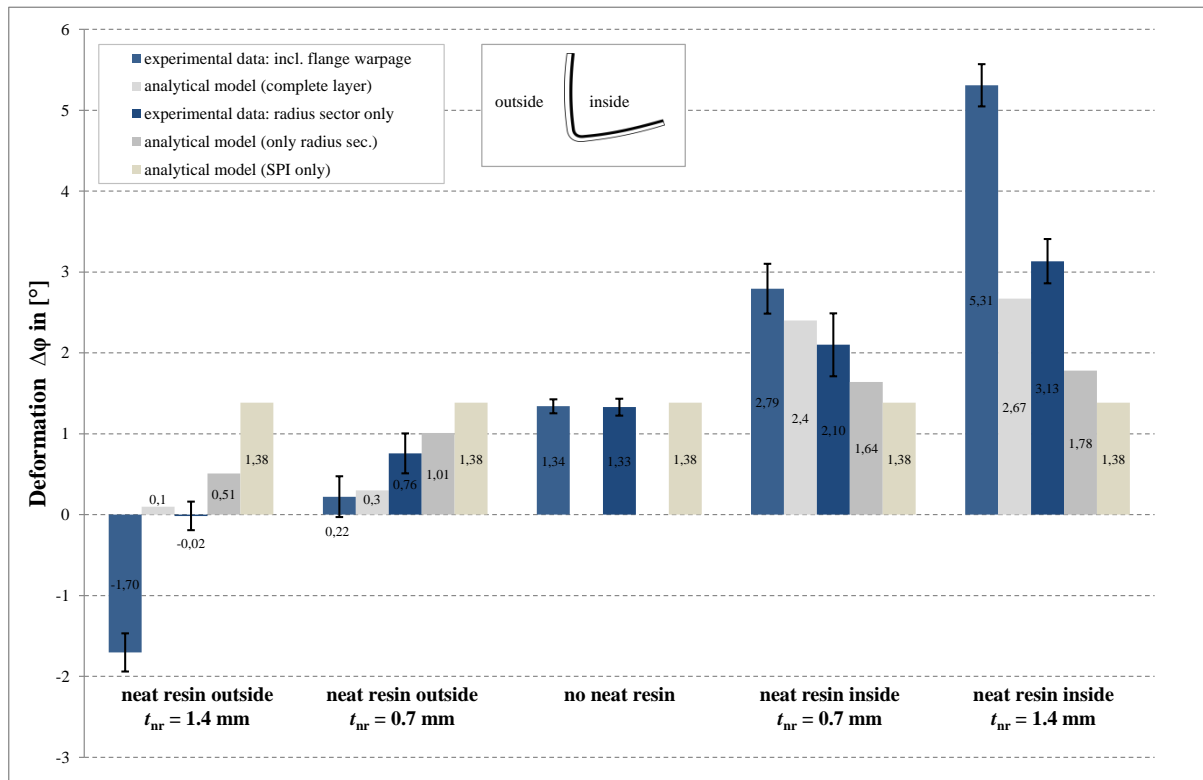
Figure 5: Experimental data. The influence of neat resin layers of different thicknesses on process induced distortions is investigated. The layers are applied either on the inside or on the outside of the L-shaped part. Deformation measurement is conducted close to the radius to account for the additional distortions of the curved area. Measurements are also conducted including the whole flange area to account for the deformation behaviour of the entire part. The experimental data is compared to the results of the analytical modelling.
