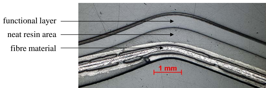
Figure 1: Cross-sectional view of a state of the art automotive CFRP-part. The part is produced in a closed mould RTM-process. The effect of fibre bridging and the resulting neat resin area are depicted. Besides the unwanted neat resin area an intentional functional layer can be seen. Source: AUDI AG.
