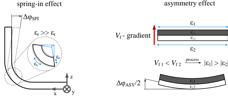
Figure 3: Underlying mechanisms for process induced deformations in RTM-FRP-manufacturing: On the left hand side a schematic of the spring-in effect resulting from anisotropic shrinkage during processing is shown. On the right hand side additional deformations due to a V_f -gradient in thickness direction leading to asymmetry. The layer with lower V_f contracts more during processing than a layer with a higher V_f which results in a curvature of the entire affected part area. The strains in both mechanism occur due to thermal and chemical shrinkage during processing.
