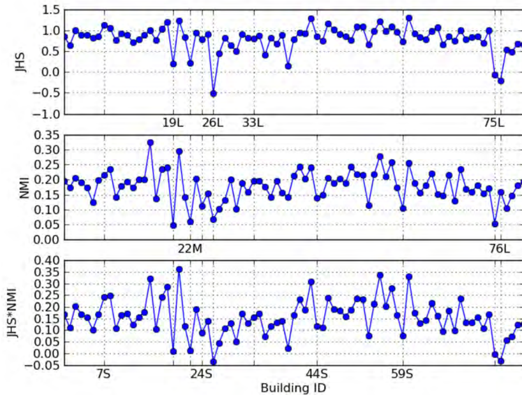
Fig. 6.24: Comparison operators NMI, JHS, and \text{NMI} \times \text{JHS} of the 81 buildings (the vertical lines mark the ten changed buildings related to Table 6.8).
