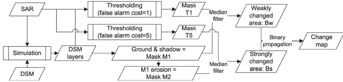
Fig. 6.4: Flowchart of pixel-based detection of positive changes between LiDAR and SAR data.
