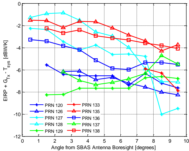
Figure 6: Comparison of the signal strength among SBAS satellites. WAAS is red, EGNOS is blue, GAGAN is cyan and MSAS is green.
