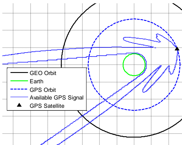
Figure 1: Typical visibility of a GNSS satellite to a user in GEO, based on a 33 dB-Hz availability threshold and the GPS transmit gain pattern from Czopek and Schollenberger (1993)
