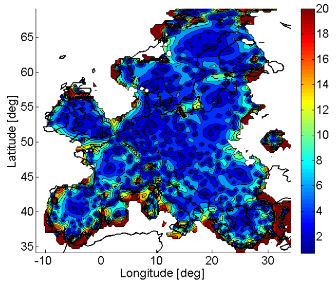
Figure 7. HDOP at 20.000 ft. with DME and HAPS
