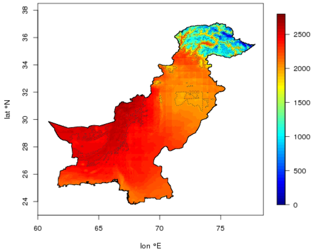
Figure 1: Annual average sum of DNI (2001-2005) in \text{kWh/m}^2 based on DLR satellite model.
