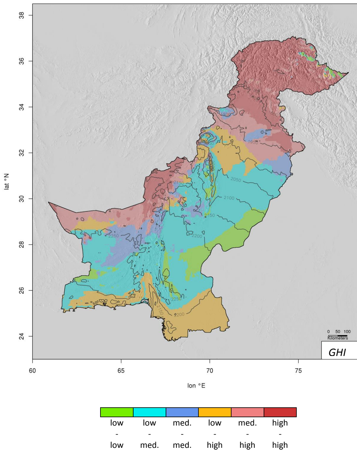
Figure 4: Color-coded solar regimes and GHI sums in (KWh/m 2 ) indicated by contour lines. Contours only showing values exceeding 1800 kWh.
