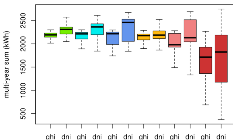
Figure 6: Distribution of multi-year-mean sums of GHI/DNI within the solar regimes (no outliers are drawn)
