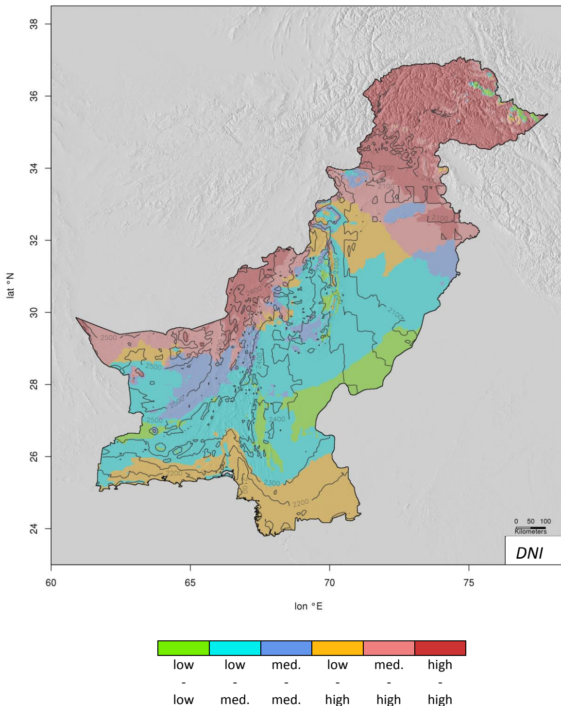
Figure 5: Color-coded solar regimes and DNI sums in (KWh/m 2 ) indicated by contour lines. Contours only show values exceeding 2000 kWh.
