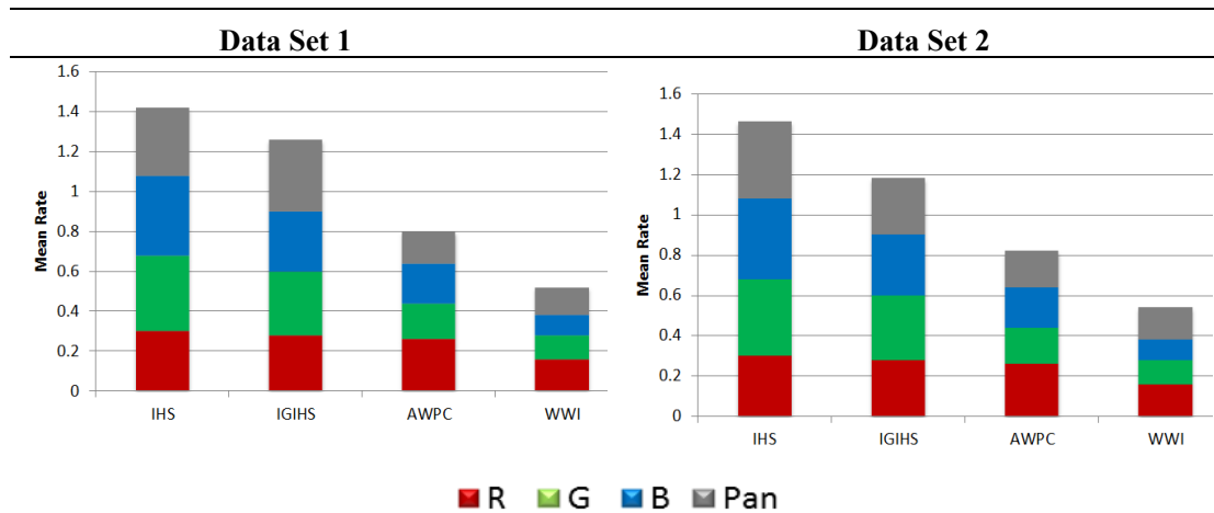
Figure 12. Comparison results of all pan-sharpening methods in both data sets.
