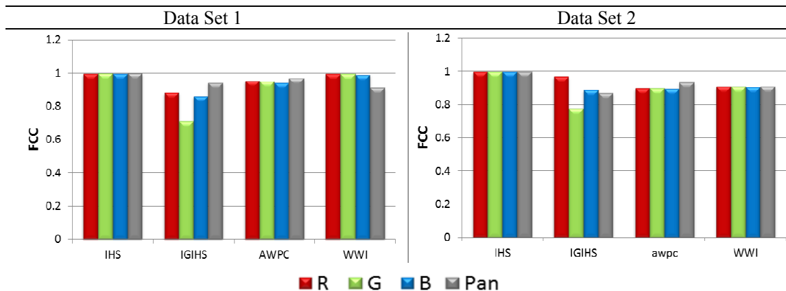
Figure 6. Results of FCC spatial quality assessment metric.
