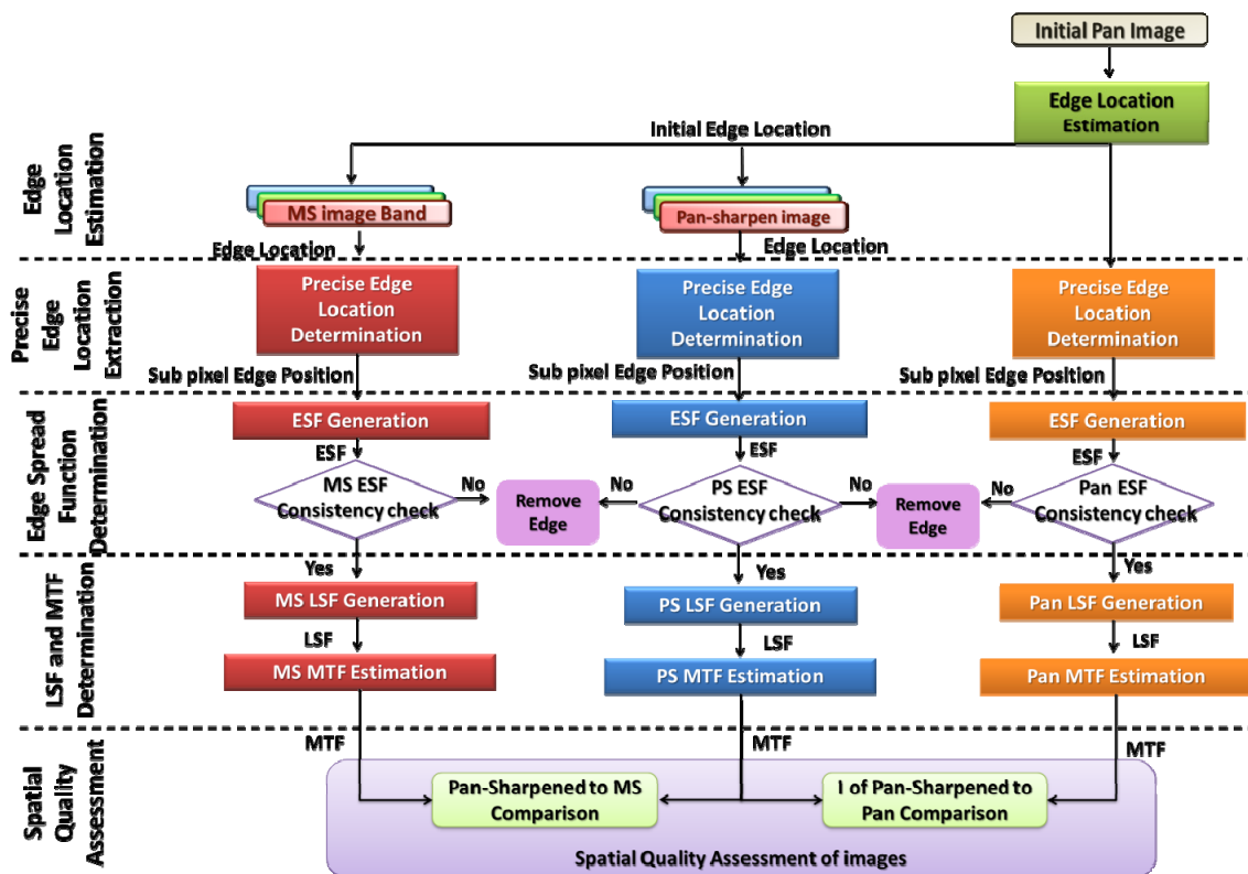
Figure 1. Diagram of the proposed edge-based quality assessment technique.
