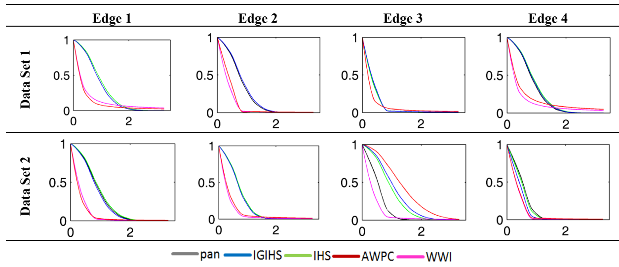
Figure 11. MTF curves, pan-sharpened and pan-image, x-axis shows the frequency and y-axis the MTF value.
