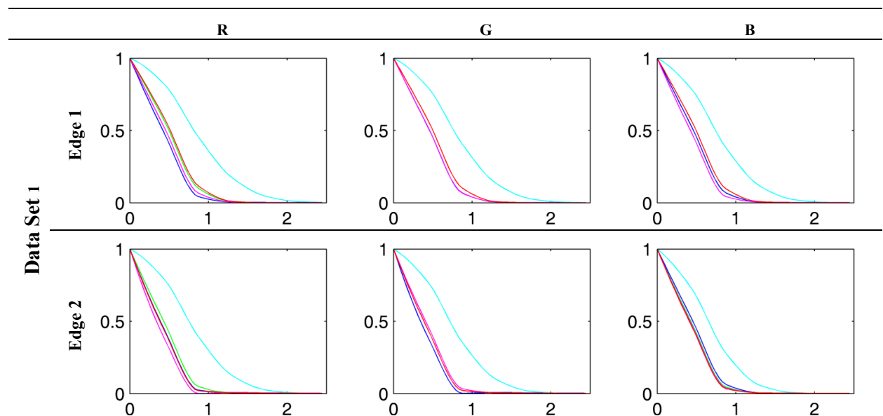
Figure 10. MTF curves, pan-sharpened and reference MS image, x-axis shows the frequency and y-axis the MTF value.
