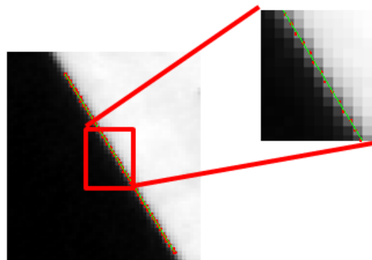
Figure 2. Sub-pixel edge location and least square line fitting process.
