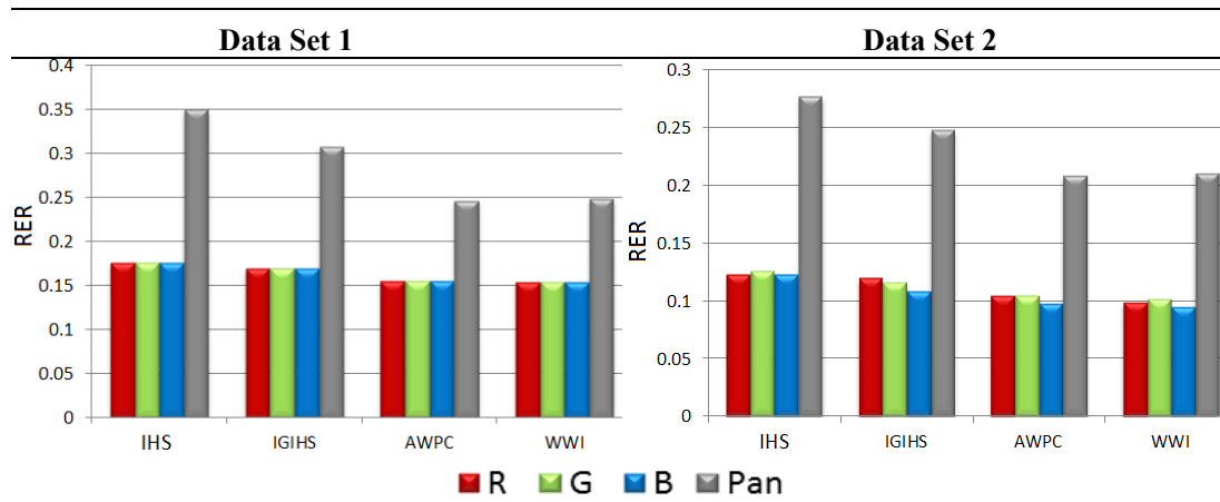
Figure 13. RER based Quality assessment of all pan-sharpening methods in both data sets.
