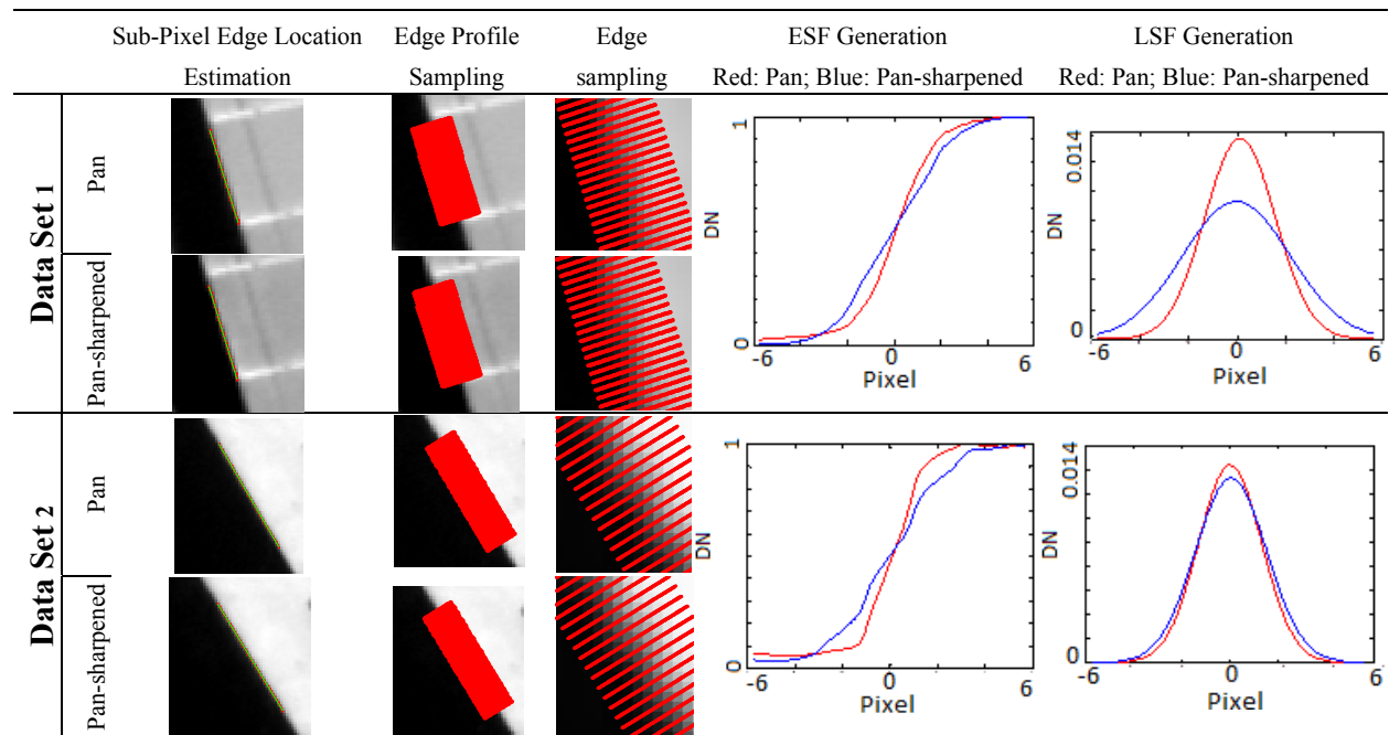
Figure 9. Samples of proposed MTF estimation strategy from sub-pixel edge locations estimation to LSF calculation in both data sets.
