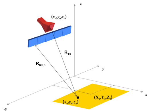
Figure 1. DBF SAR with ULA in along track
