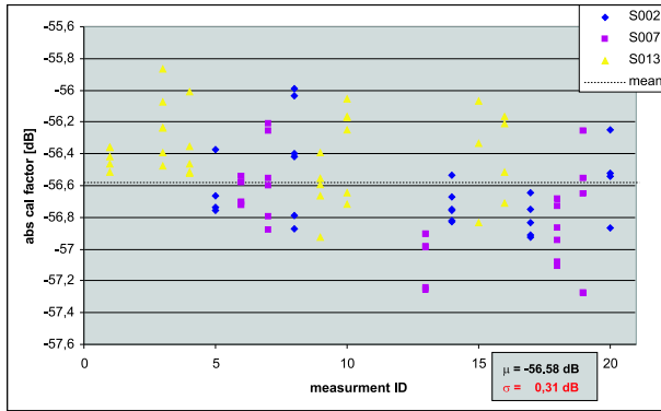
Figure 7: Absolute calibration factor versus measurement ID derived from all reference targets deployed and all StripMap beams being measured.
