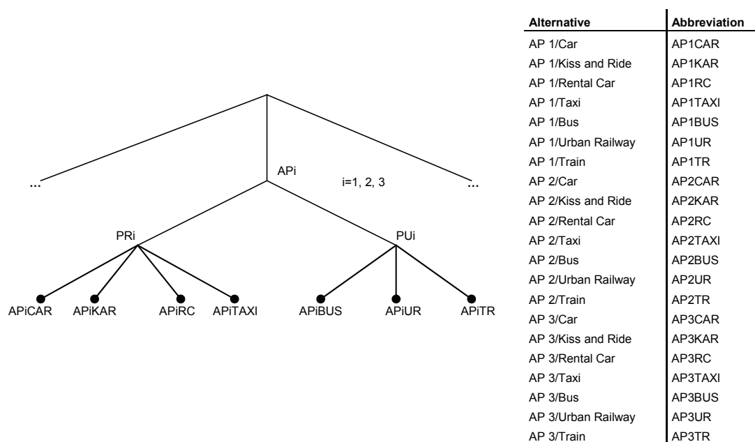
Figure 4.07: Nesting Structure
