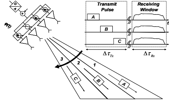
Fig. 5: Intra-pulse beamsteering in elevation
