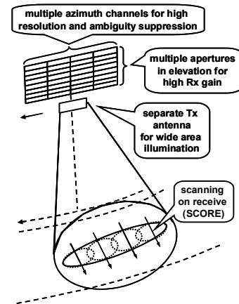
Fig. 1: High resolution wide swath (HRWS) SAR [4].
