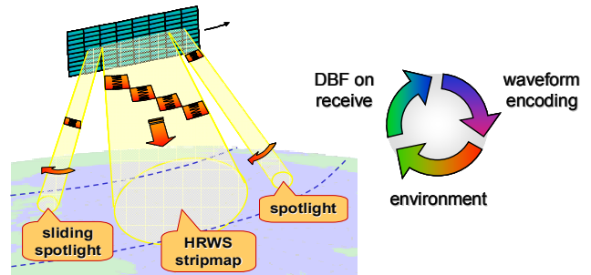
Fig. 7: Hybrid and adaptive SAR imaging modes.
