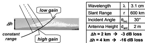
Fig.. 3: Gain loss from topography during pulse chasing
