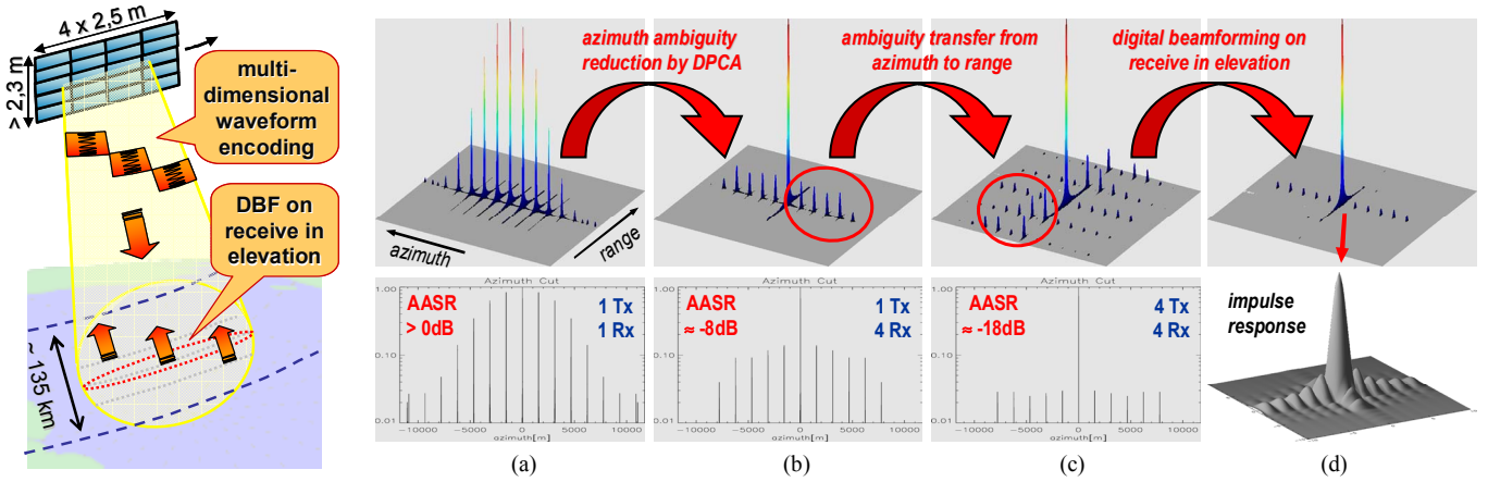
Fig. 6: Multidimensional waveform encoding in azimuth. Left: Staggered illumination by multiple narrow azimuth beams. Right: Transfer of ambiguous energy from azimuth to range. (a) impulse response from one transmitter and one receiver. (b) azimuth ambiguity suppression by four receive channels. (c) ambiguity transfer from azimuth to range by intra-pulse azimuth beamsteering. (d) range ambiguity suppression by digital beamforming on receive.
