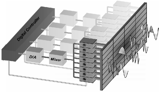
Fig. 4: Transmitter for 3-D spatio-temporal radar pulse encoding with four azimuth waveform generators and intra-pulse elevation beam-steering.
