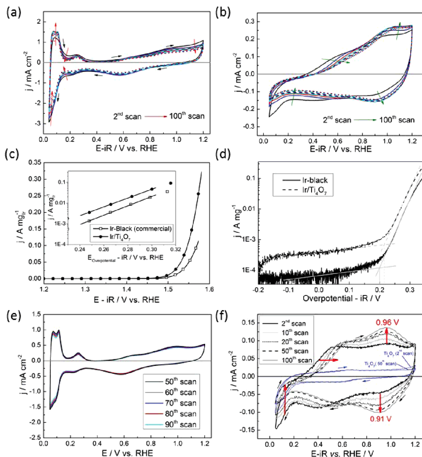
Fig. 8. Cyclic voltammetric curves of (a) Ir-black and (b) Ir/Ti 4 O 7 deposited on the GC-RDE, measured at a sweep rate of 50 mV s -1 . (c) Mass activities of Ir-black and Ir/Ti 4 O 7 catalysts for the OER measured at a sweep rate of 5 mV s -1 and rotation speed of 2500 rpm. The inset shows the corresponding Tafel slopes. A comparison of the j - E characteristics without normalization is shown in (d). Cyclic voltammetric curves of (e) Ir-black and (g) Ir/Ti 4 O 7 after the OER measurements with different temperatures from 25 °C to 70 °C. All the experiments were carried out in Ar-saturated 0.5 M H 2 SO 4 at 25 °C.
