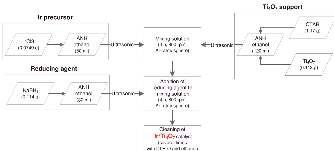
Fig. 1. Scheme of the synthesis procedure for 30 wt% Ir/Ti 4 O 7 catalyst. DI = deionized water, ANH = anhydrous, CTAB = cetyltrimethylammonium bromide.
