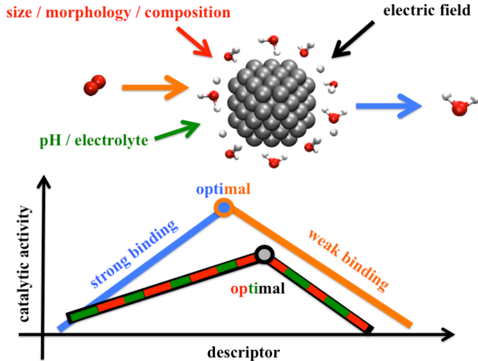
Figure 2: Schematics of Sabatier-type volcano plots. The blue and orange lines represent the usual approach based only on the adsorption strength of the adsorbates to the catalyst surface. The black-green-red lines represent the real situation in which several other effects (catalyst composition and morphology, environment) are taken into account in addition to binding in order to provide realistic predictions.
